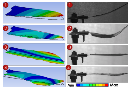
Figure 9: Modal Analysis: Nature of mode shapes.
