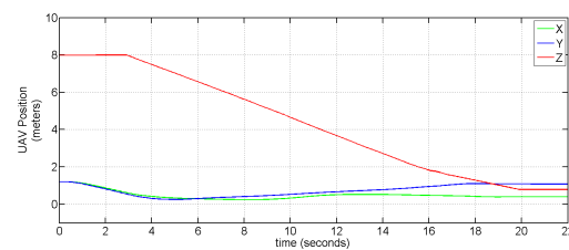
Figure 17: Evolution of the quadrotor position in x,y,z axis in the autonomous landing test on a moving platform.
