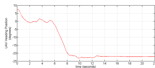
Figure 18: Evolution of the absolute heading of the quadrotor in the autonomous landing test on a moving platform.
