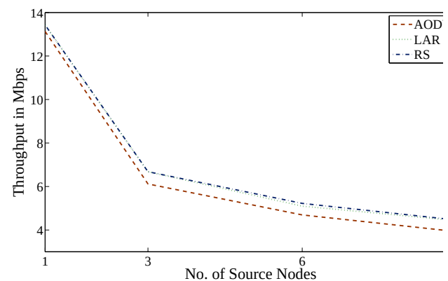
Figure 10: Achieved network throughput using free space channel propagation model for the mission scenario
