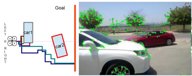
Figure 9: The path of the AR.Drone avoiding two cars (left), based on the processed image (right)
