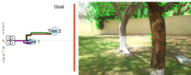
Figure 4: The path of the AR.Drone failing to avoid two obstacles (left) based on the image without ForeGround classification(right)
