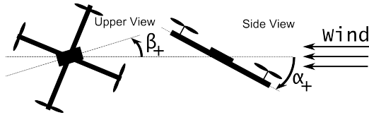
Figure 10: Positive Yaw and Pitch angles
