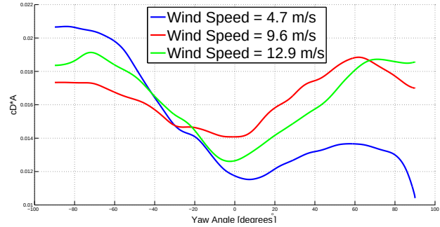
Figure 14: c_{DA}(\beta) at different wind speeds
