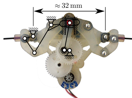
Figure 2: Flapping mechanism prototype and its kinematic representation.
