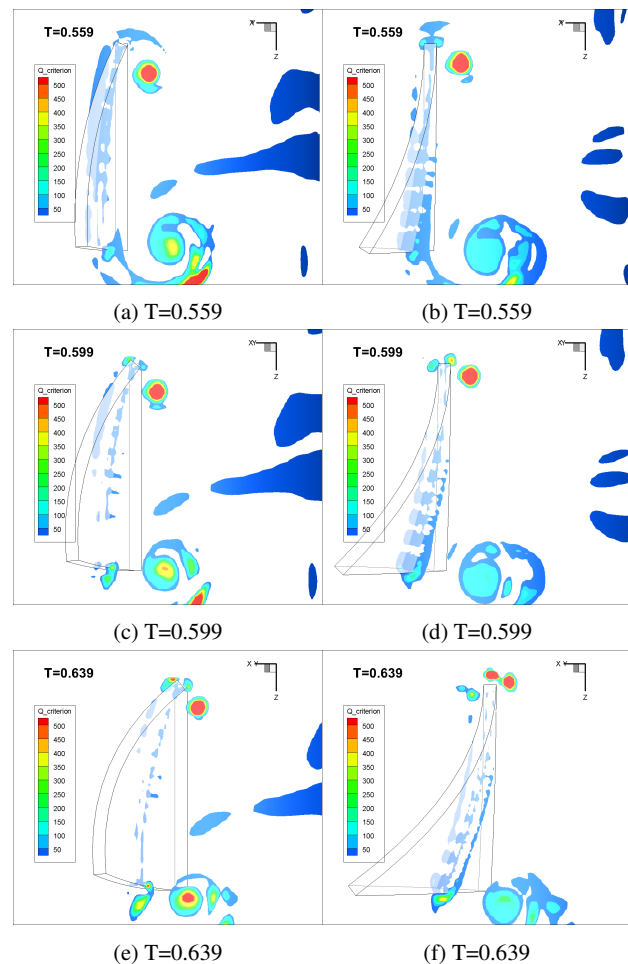
Figure 6: Q criterion contour plots of the deforming end and deforming center cases during the instroke, with the wings moving to the right. The deforming center case on the left and the deforming end case on the right.
