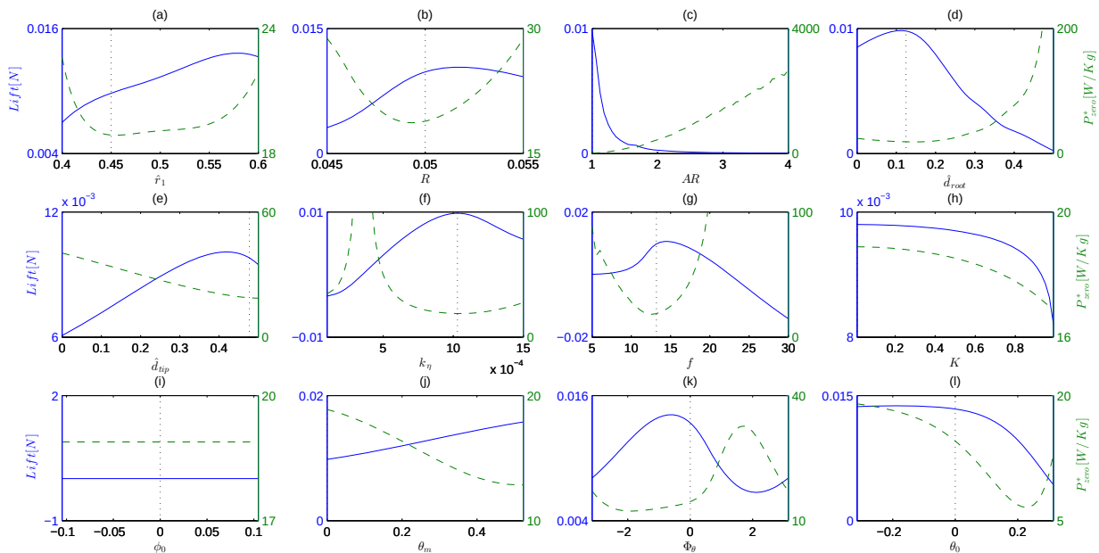
Figure 7: Effect of single parameters on the power pattern P_{\text{per}}^* while \phi_m = \pi/3 . Details as in Figure 6.
