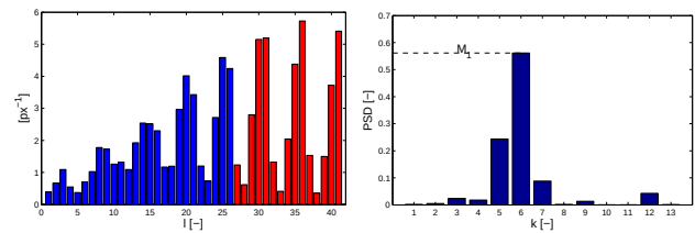
Figure 9: Cross-correlation of the histogram and a series of correlation, rescaled w.r.t. the gaussians. The part with the total power density after removal of the DC component. Behavior is colored red.
