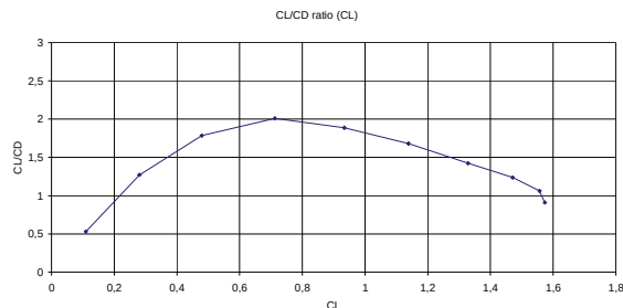
Figure 10: C_L/C_D ratio as function of C_L
