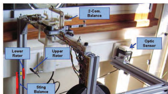
Figure 8: Experimental Set up of Tilt-Rotor in NACR project.
