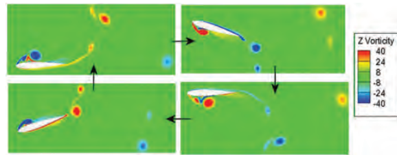
Figure 4: Vorticity contour plot of the single airfoil
