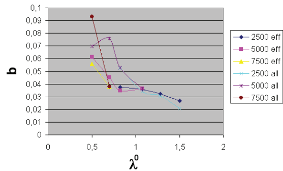
Figure 12: Coefficient b as function of \lambda_{0.75} for AV-31 propeller for various RPM.
