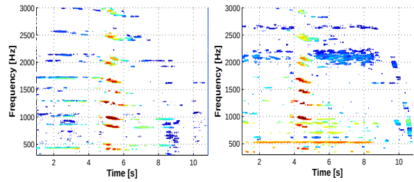
Figure 6: Spectrogram sound intensity X direction. Left: horn. Right: horn and propeller.
