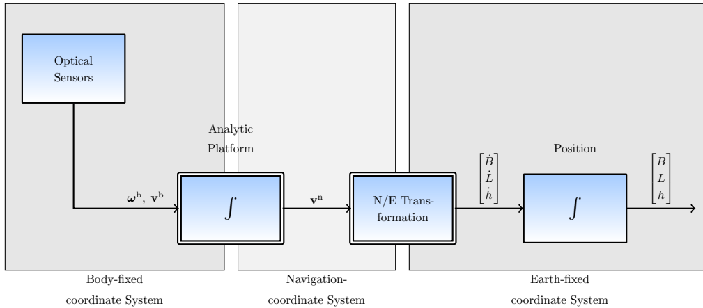
Figure 4. Simplified strap-down algorithm for the proposed optical navigation system
