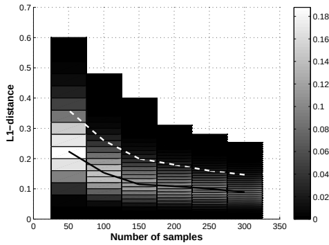
Figure 4: Relation between the number of samples used in random sampling and the accuracy of the estimate. The y-axis shows the L1-distance between the estimated and the true distribution, the x-axis shows the number of samples, s = \{50, 100, 150, 200, 250, 300\} . The intensity represents the probability, where white indicates high probability and black a low probability. The black line indicates the mean distance from the actual distribution, the white dashed line the 95 th percentile of the distribution.
