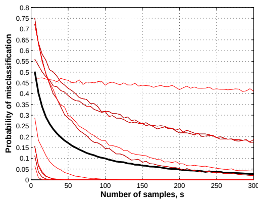
Figure 15: Misclassification due to random sampling, H = 5 . Thick black line: average error when sampling from the learned distributions. Thin red lines: average errors for ten images from the height control experiment. See Subsection 6.4 for an explanation.
