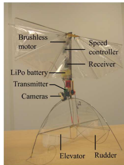
Figure 10: The 15-gram ornithopter used for the height control experiments.
