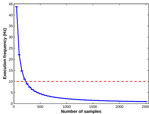
Figure 3: Mean execution frequencies and corresponding standard deviations of a MATLAB-implementation of TMG for a number of samples s from 50 to 2500 (blue solid line). The 10 Hz limit is shown by a red dashed line.
