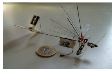
Figure 1: The DelFly Micro is a 3.07-gram ornithopter with a wing span of 10 cm. Autonomous flight will require fast image processing with little computational power available.
