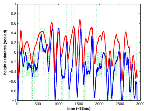
Figure 9: Comparison of the helicopter's y-coordinate in the external camera (solid line, scaled to [-1, 1] with 1 being the top of the image), and the height estimated by the algorithm (grey line, scaled to [-1, 1] with h = 3 mapped to 0). The black dashed line is a smoothed version of the grey line.
