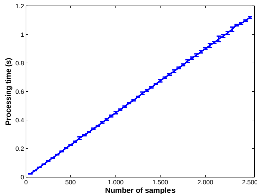
Figure 2: Mean processing times of a MATLAB-implementation of TMG for a number of samples s from 50 to 2500. The error bars indicate the standard deviation.
