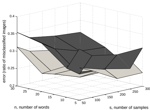
Figure 7: Mean error (expressed as the ratio of misclassified images) when using colour images (dark grey) and when using black-and-white images (light grey) for s \in \{50, 100, 200, 300\} and n \in \{5, 10, 20, 30\} .
