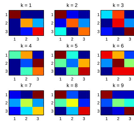
Figure 17: Confusion matrices for the texton method with n = 30 and s = 300 for nine different rooms.
