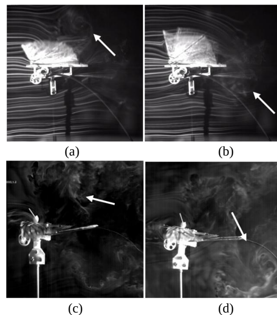
Figure 9: Flow Visualization for the original wing and biomimetic wings
