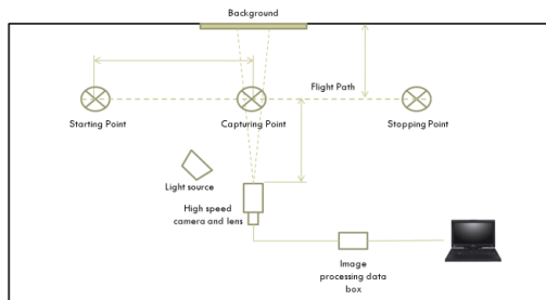
Figure 5: Free flight setup.
