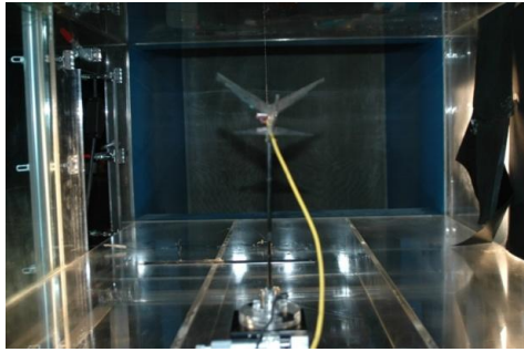
Figure 3: Wind tunnel experiment setup
