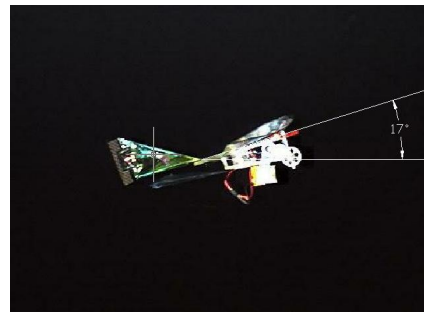
Figure 8: Free Flight Test Result for original wing
