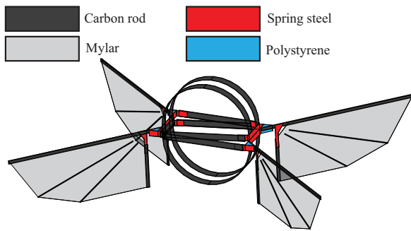
Figure 8: The total structure showing materials used
