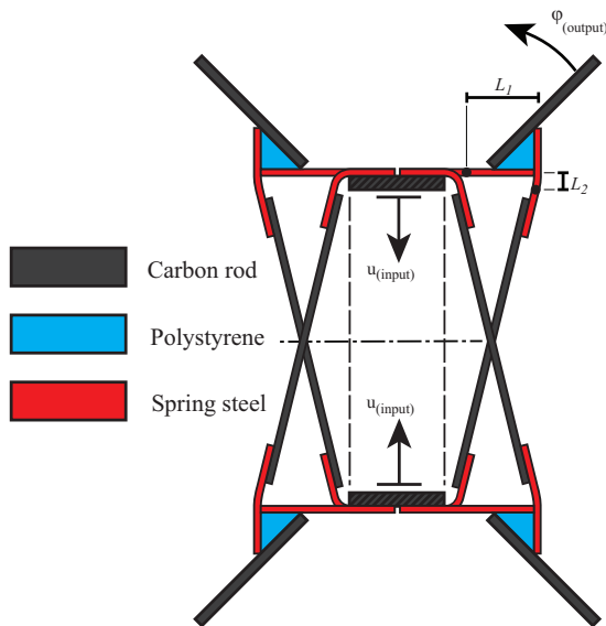
Figure 2: The compliant mechanism used to drive the wings
