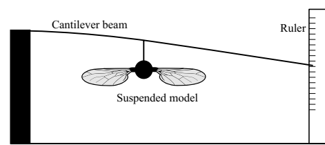
Figure 10: Test setup for measuring lift production of the suspended model
