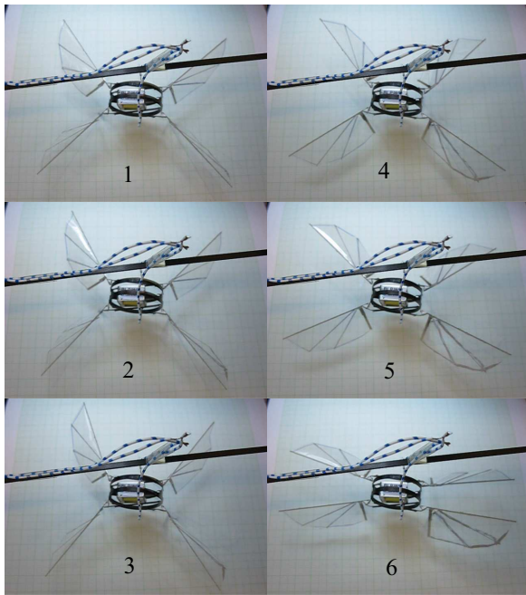
Figure 11: Sequence of pictures showing the the development of wing sweeping and pitching during one flapping cycle
