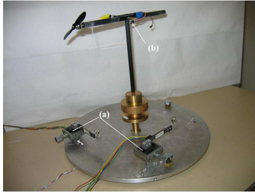
Figure 15: Nano bench version 2 (a) Micrometer screws (b) Wires passing through the carbon tube
