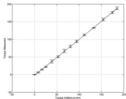
Figure 10: Torque calibration of micro test bench
