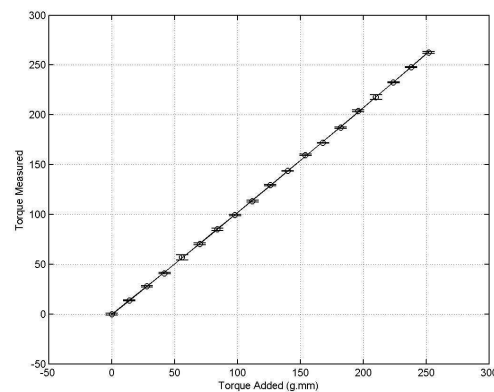
Figure 14: Torque calibration of nano bench version 1
