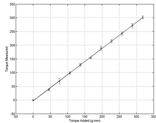
Figure 18: Torque calibration of nano bench version 2
