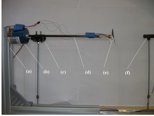
Figure 20: Torque sensor (a)Supporting base (b)Torque sensor (c) Laser emitter (d) Horizontal supporting beam (e) Motor and rotor (f) Laser detector
