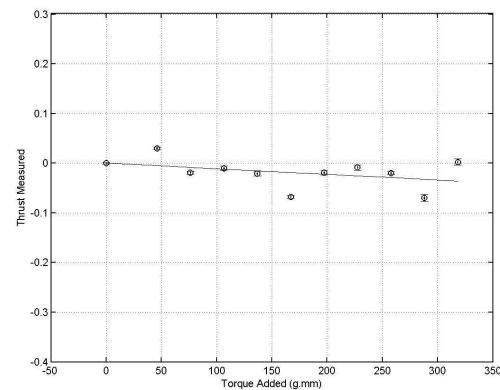
Figure 19: Influence of torque to thrust
