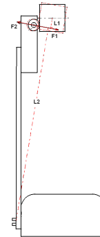
Figure 5: Principle of the torque measurement
