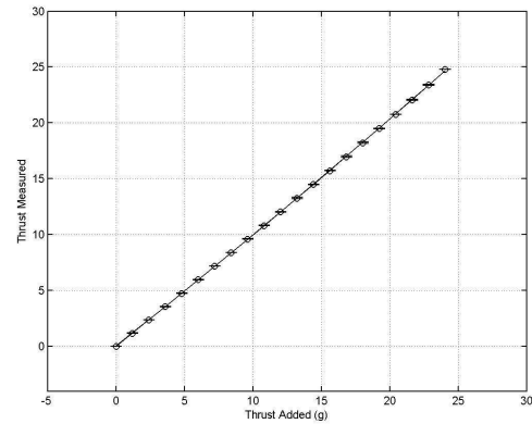
Figure 13: Thrust calibration of nano bench version 1
