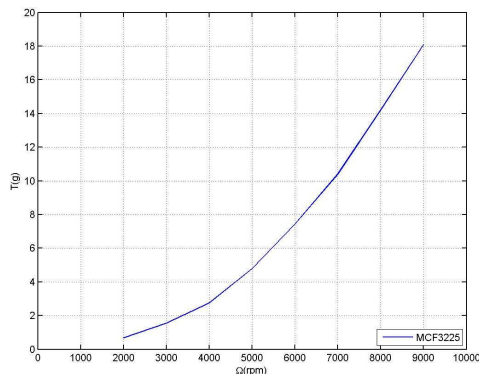
Figure 2: Thrust vs. rotational speed
