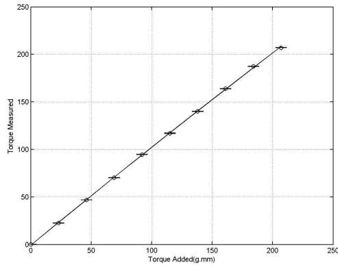
Figure 21: Torque calibration of torque sensor
