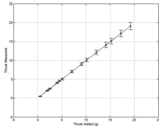
Figure 6: Thrust calibration of test bench 1
