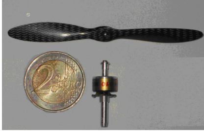
Figure 1: Micro motor and rotor MCF3225
