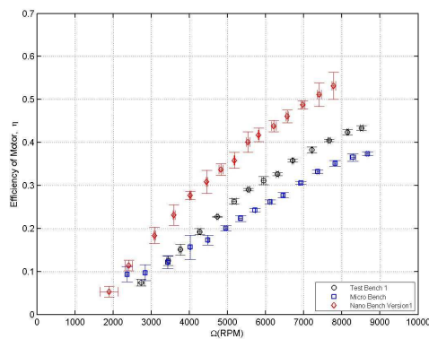
Figure 25: Motor efficiency at different rotational speeds
