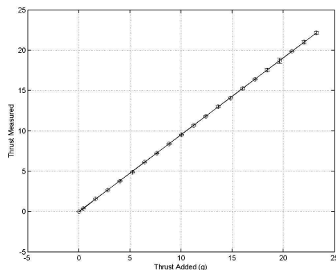
Figure 16: Thrust calibration of nano bench version 2
