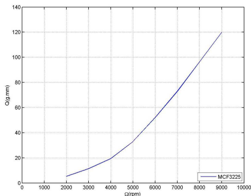
Figure 3: Torque vs. rotational speed
