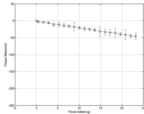
Figure 17: Influence of thrust on torque
