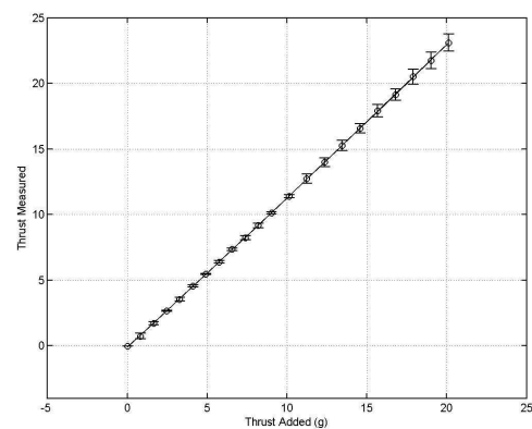
Figure 9: Thrust calibration of micro test bench
