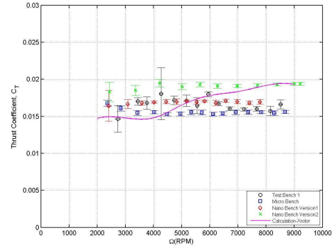
Figure 22: Thrust coefficient at different rotational speeds
