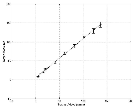
Figure 7: Torque calibration of test bench 1
