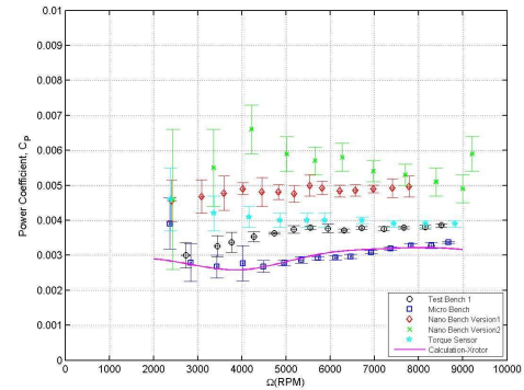
Figure 23: Power coefficient at different rotational speeds
