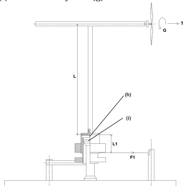
Figure 12: Section view of nano bench version 1 (h) Upper wedge (i) Lower wedge
