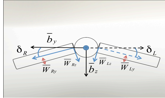
Figure 3: Front View - \delta_R and \delta_L
