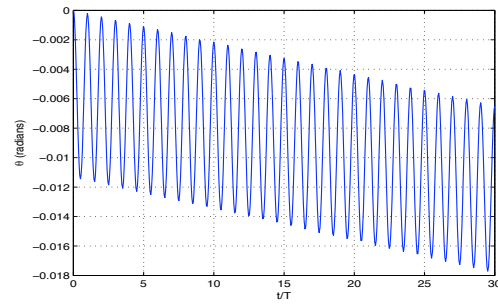
Figure 9: Pitch angle, \theta , of central body
