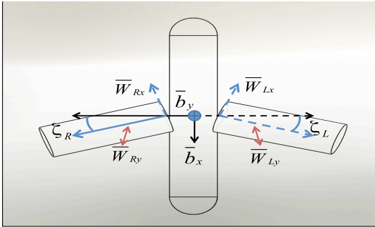
Figure 5: Top View - \zeta_R and \zeta_L
