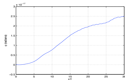
Figure 10: Roll angle, \phi , of central body
