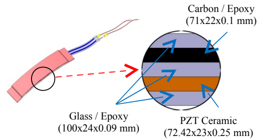
Figure 4: Piezo-composite actuator.
