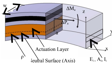
Figure 1: Schematic of the curvature change of a laminated beam with electro active layer.
