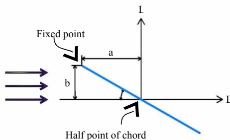
Figure 3: Moment of fixed wing section.
