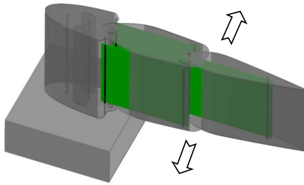
Figure 6: Structural application model using piezo-composite actuator
