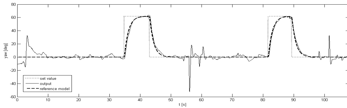
Figure 13: Time history of yaw angle \psi [deg]
