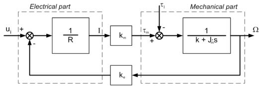
Figure 8. Block diagram of a DC-motor dynamics.
