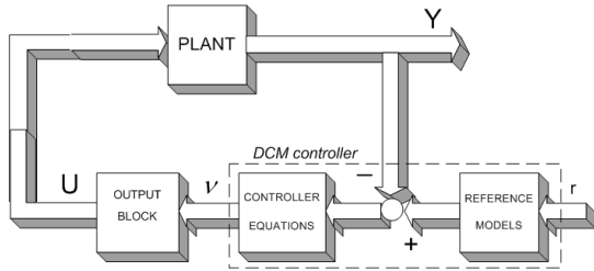
Figure 2: Block diagram of a control system.
