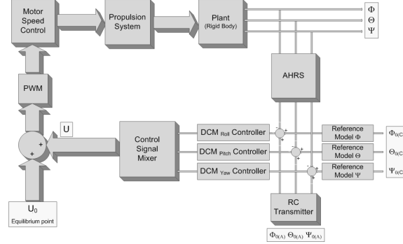
Figure 10: Control implementation.
