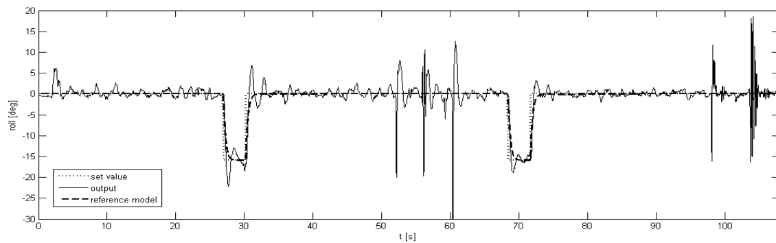
Figure 11: Time history of roll angle \phi [deg]
