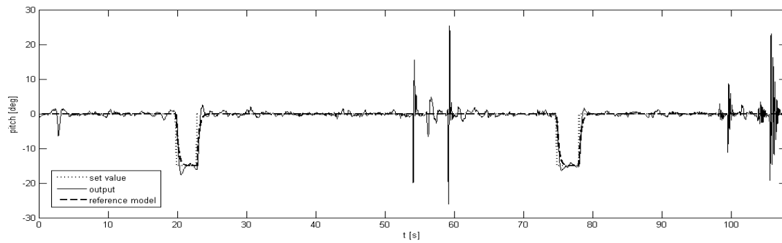
Figure 12: Time history of pitch angle \theta [deg]
