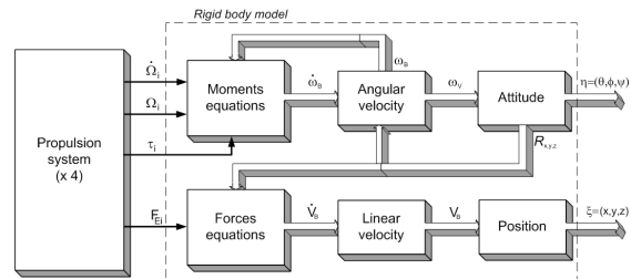
Figure 7: Block diagram of the rigid body model.
