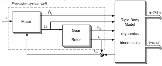
Figure 6: Block diagram of a system dynamics.
