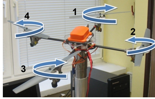
Figure 4: Quadrotor concept motion description.
