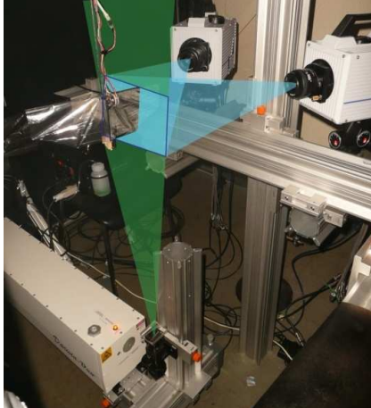
Figure 2: Experimental set-up for Stereoscopic Particle Image Velocimetry
