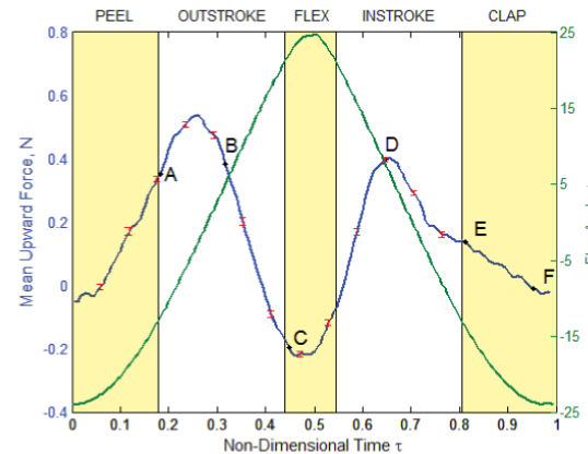
Figure 5: Upward force fluctuations and flapping angle during one flap cycle. Error bars show standard deviation. Labels A to F correspond to the red-colored wing sections identified in fig. 4
