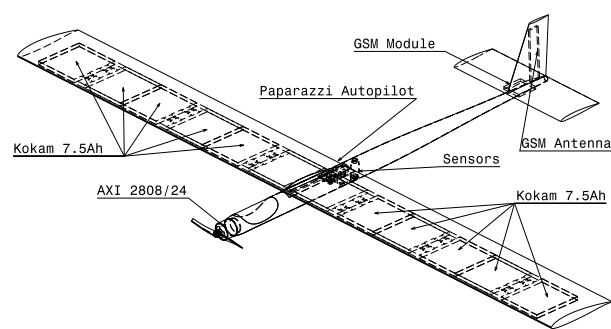
Figure 8: Sketch of the prototype with its components.
