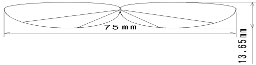
Figure 4. Flapping wing shape
