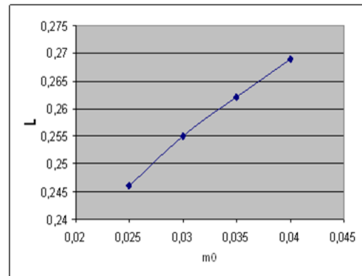
Figure 4: Wing span vs. m_0 for optimal design.
