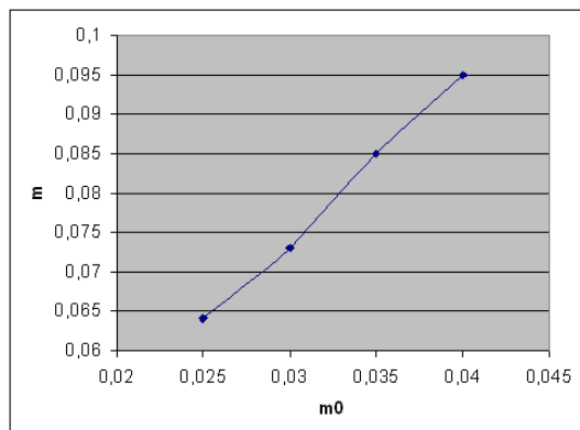
Figure 3: Total mass vs. m_0 for optimal design.
