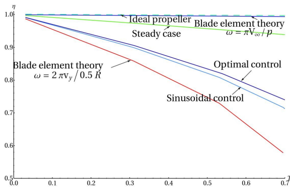
Fig.12 Efficiency comparison for p/l=1
