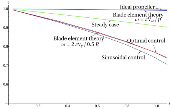
Fig.11 Efficiency comparison for p/l=2
