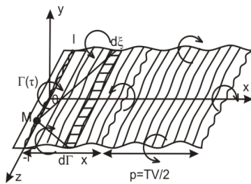
Fig.7 Vortex sheet investigated
