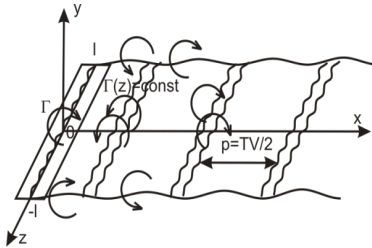
Fig.3 Simplified model for nonstationarity influence investigation
