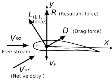
Fig. 2 Diagram of the forces on the flapping wing
