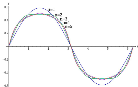
Fig.8 Function of optimal control obtained; n=1,2,3,4,5
