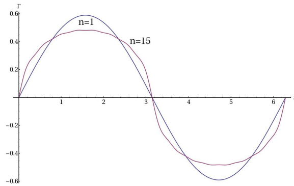
Fig.9 Function of optimal control obtained; n=1,15
