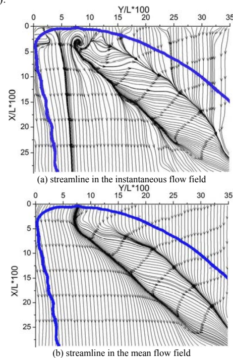
Figure 8: streamline in flow field on the plane through the primary leading-edge vortex core ( \alpha = 8^\circ ) (the blue solid line is the outline of the butterfly model)
