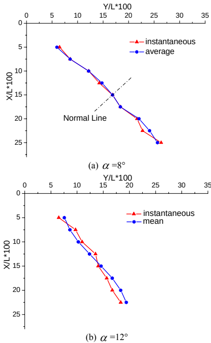
Figure 9: position of the primary leading-edge vortex axis
