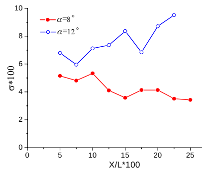
Figure 11: turbulence intensity of the axial velocity
