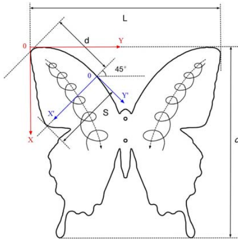
Figure 2: sketch of simplified Papilio ulysses (Besides the butterfly model, the sketch contains the leading-edge vortices and two rectangular coordinate systems for dye visualizations and PIV measurements)
