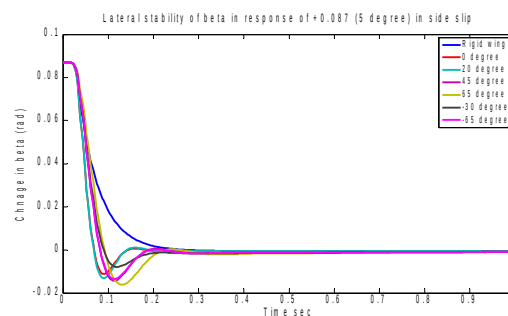
Fig. 11. Lateral stability results of the MAV (change in \beta )
