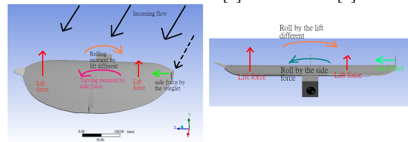
Fig. 19. Asymmetric winglet MAV during the turn. (front view at right)
