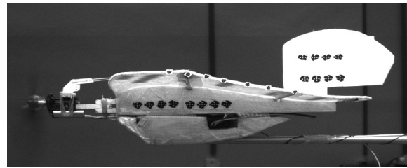
Fig. 6. The aeroelasticity test of the MAV in wind tunnel. Note. The marker system are provided by Fraunhofer ITB Germany.
