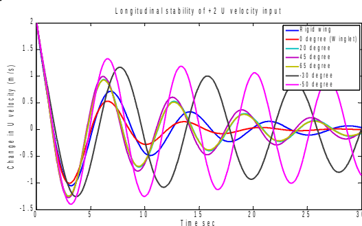
Fig. 9. Longitudinal stability results of the MAV (change in U velocity)
