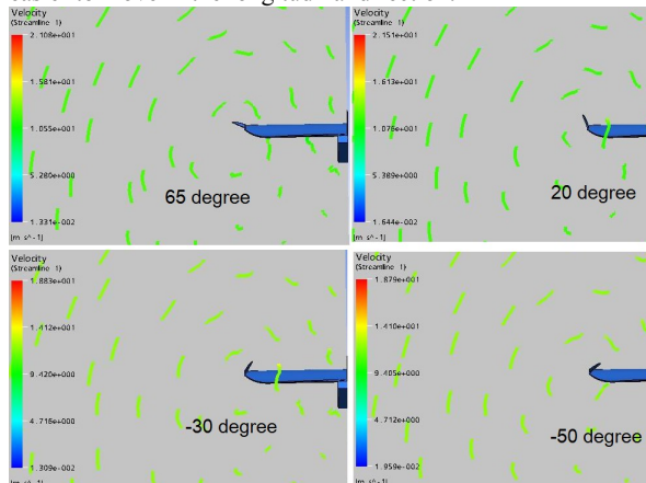
Fig. 18. The stream line of MAV with different angle of winglet. Note: the location of the vortex center is clearly different.
