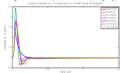
Fig. 12. Lateral stability results of the MAV (change in r )
