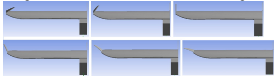
Fig. 4. CAD model of different winglet angle, from the top left to bottom right are:-50,-30,0,20,45,65 degree.
