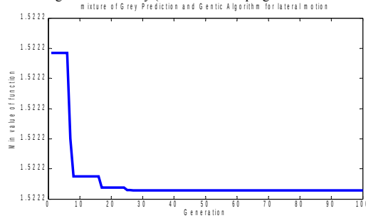
Fig. 17. Mixture of G.P and G.M search of minimum value of the function for lateral stability (base on the damping ratio of the motion)
