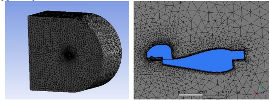
Fig. 7. Left, mesh of the flow region. Right, mesh around the MAV.
