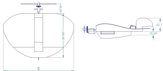
Fig. 2. The dimension of the MAV. Note: all units are in mm.
