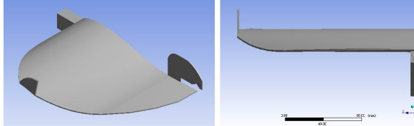
Fig. 3. Left, platform MAV with winglet (iso view). Right, back-view of the MAV with winglet.
