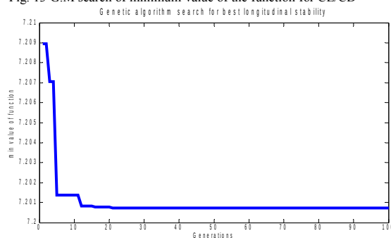
Fig. 14 G.M search of minimum value of the function for Longitudinal stability (base on the damping ratio of the motion)
