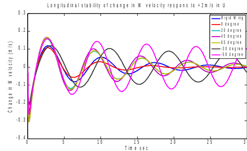
Fig. 10. Longitudinal stability results of the MAV (change in W velocity)
