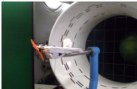
Fig. 5. Wind tunnel test model
