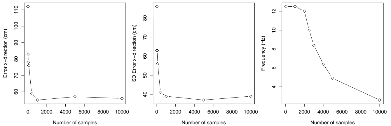
Figure 5: Speed versus accuracy trade-off in x -direction as a function of the number of used samples in the histogram extraction step.
