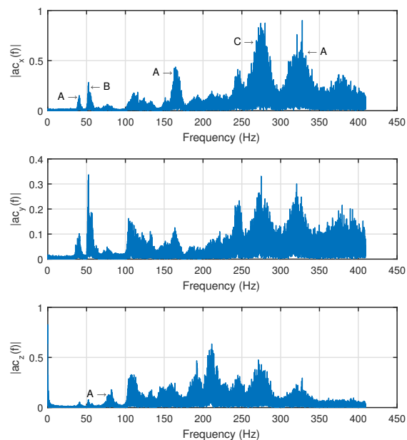
Figure 4: Vibration of T-Lion UAV measured by ADIS IMU
