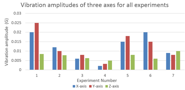
Figure 9: Kyosho Zeal sheet test results on three axes of UAV
