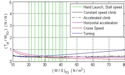
Fig .2. Constraint analyses for the IUT MAV2013
