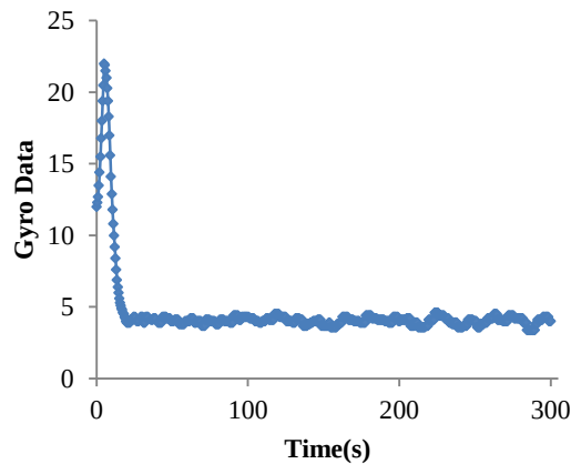
Fig. 7. Flight Test No. 3
