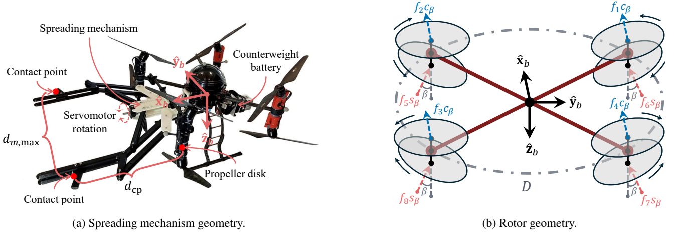
Figure 2: FT-X8 geometry: (a) spreading direction \hat{s}_b = \hat{y}_b and (b) c_\beta = \cos \beta , s_\beta = \sin \beta .
