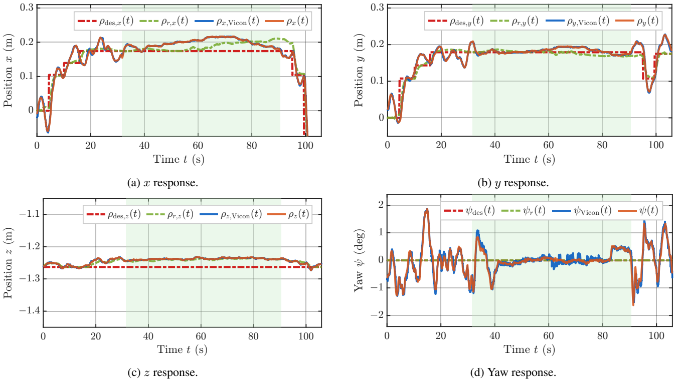
Figure 6: Vehicle motion during the spreading experiment. The shaded region marks the bilateral spreading phase.
