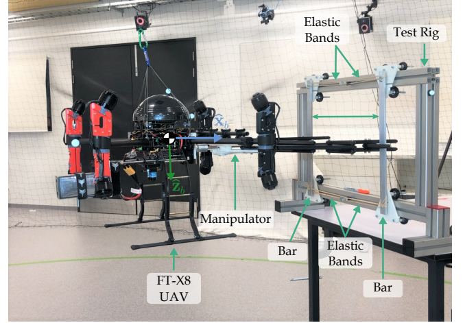
Figure 5: Experimental setup for elastic obstacle separation.
