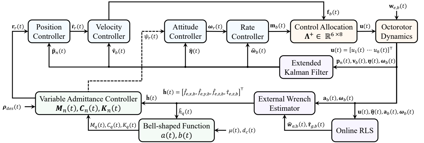
Figure 3: Variable admittance control architecture.
