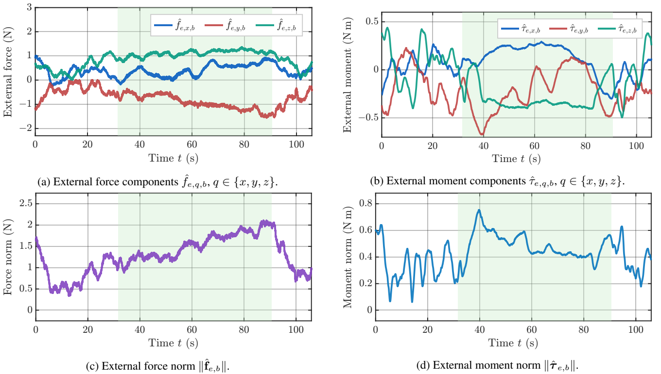
Figure 7: RLS-corrected external wrench estimate during the spreading experiment, expressed in the body frame. The component plots show the dominant interaction directions, while the norms summarize the force and moment magnitudes.
