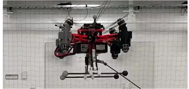
Figure 1: Contact experiment between the smaller fixed-tilt multirotor and a vertical flexible rod [13].
