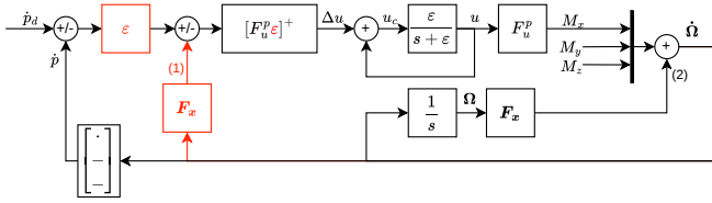
Figure 2: Structure for the gyro controller. Red signals and blocks are only present in ANDI.
