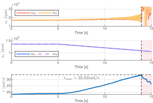
Figure 8: Motor commands and yaw rate in the loss of control test of the INDI controller. The red area indicates that loss of control has occurred.
