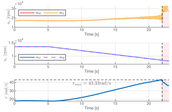
Figure 9: Motor commands and yaw rate in the loss of control test of the ANDI controller. The red area indicates that loss of control has occurred.
