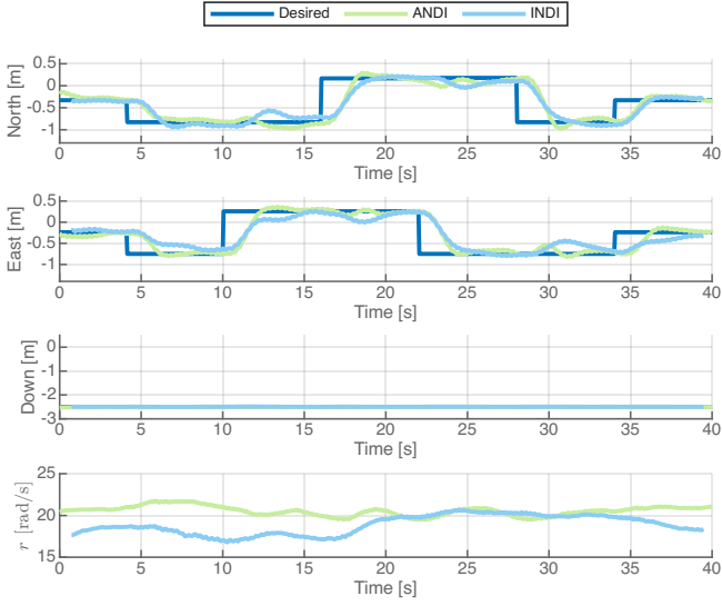
Figure 10: Position tracking comparison of a square trajectory with the INDI and ANDI controllers.
