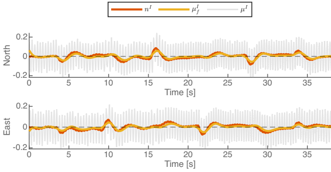
Figure 11: Principal axis of rotation tracking with the INDI controller.
