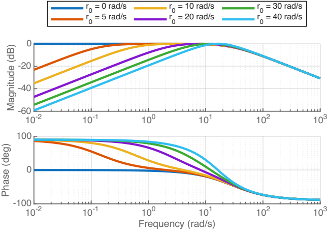
Figure 4: Bode plot of the INDI dynamics at different yaw rates.
