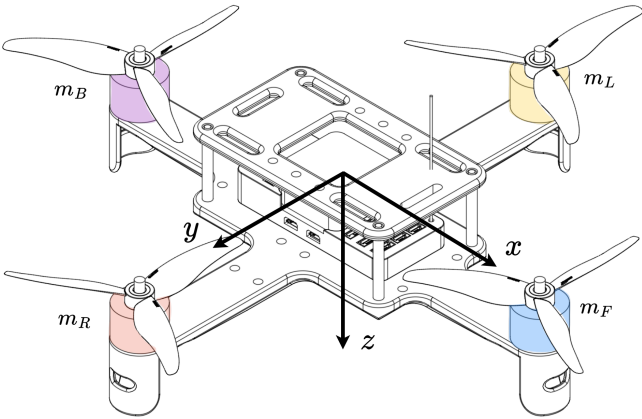
Figure 1: The quadcopter used in the experiments with body axis definition.
