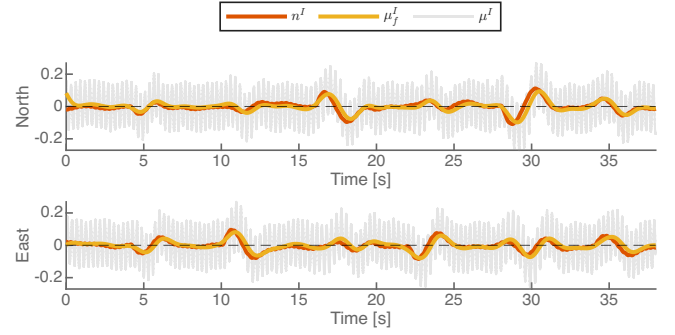
Figure 12: Principal axis of rotation tracking with the ANDI controller.
