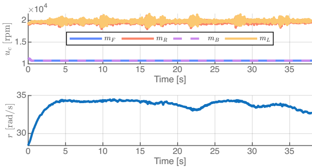
Figure 15: Command signals and yaw rate during the ANDI square tracking test at high spin rate.
