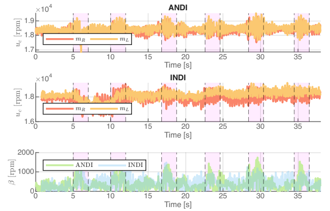
Figure 13: Comparison of control effort during the square tracking task between the INDI and ANDI controllers. Shaded areas indicate time intervals in which the drone is actively moving.
