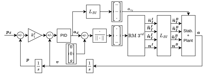
Figure 6: Guidance controller.
