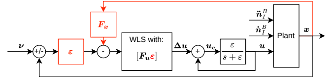
Figure 5: Allocation diagram. Red signals and variables are additional in ANDI compared to INDI.
