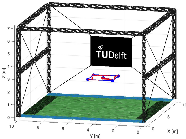
Figure 14: 3D flight path of the square trajectory using the ANDI controller at an average spin rate of 34.5 \text{ rad s}^{-1} recorded at the Cyberzoo.
