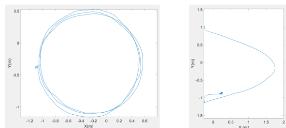
Figure 10 - Circle and Parabola
