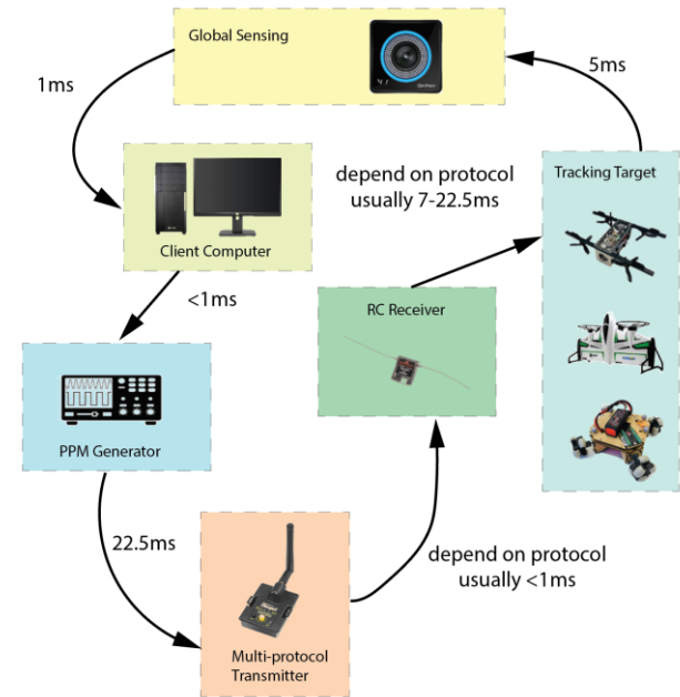
Figure 6 - System latency
