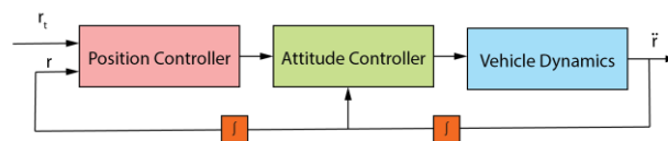
Figure 9 - Control Diagram
