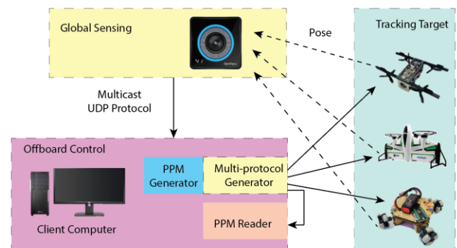
Figure 1- System Overview
