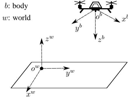
Figure 2: MAV body ( x^b, y^b, z^b ) and world ( x^w, y^w, z^w ) coordinate systems.
